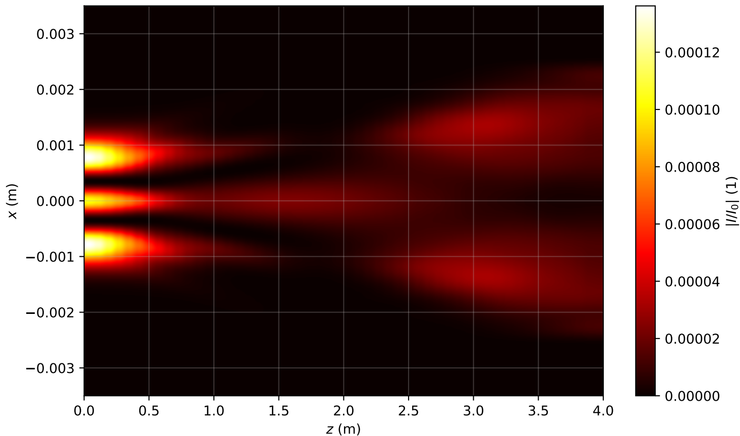
Intensity profile I(x, y = 0, z)/I_0 , P_{in}=4.0P_{cr} , artificial time
